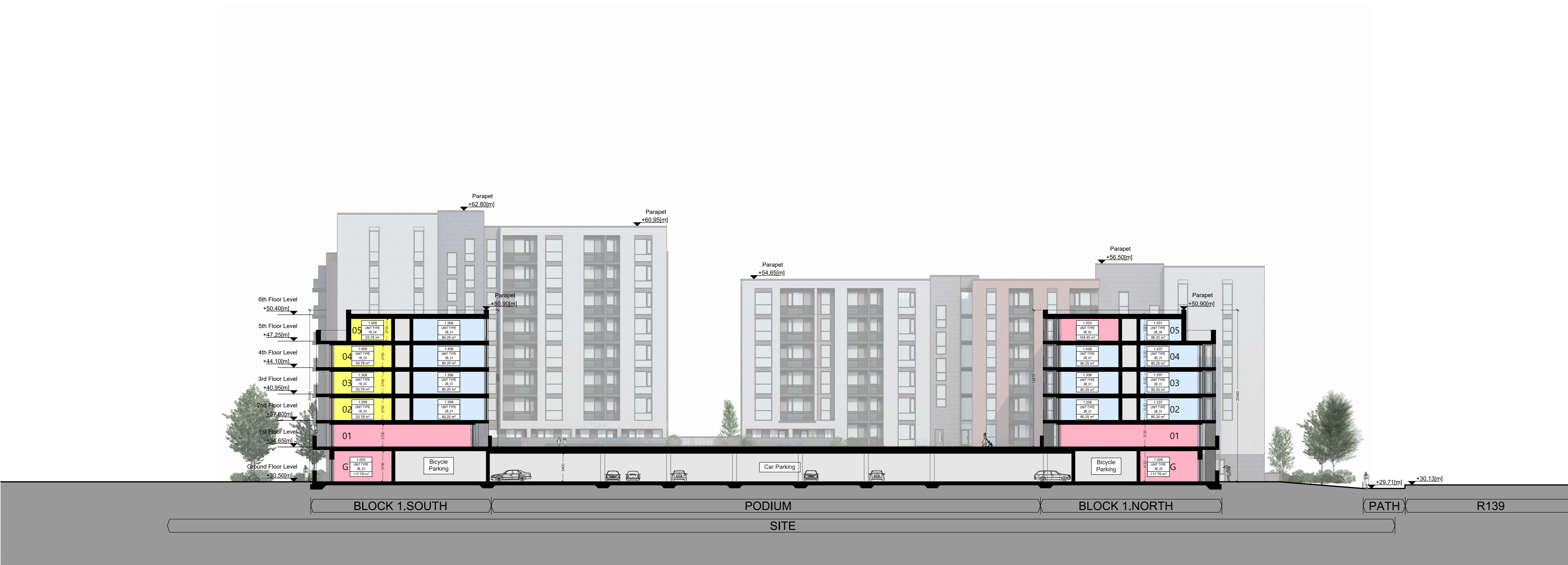
Section BB - Block 1 Scale 1:200 @A0
